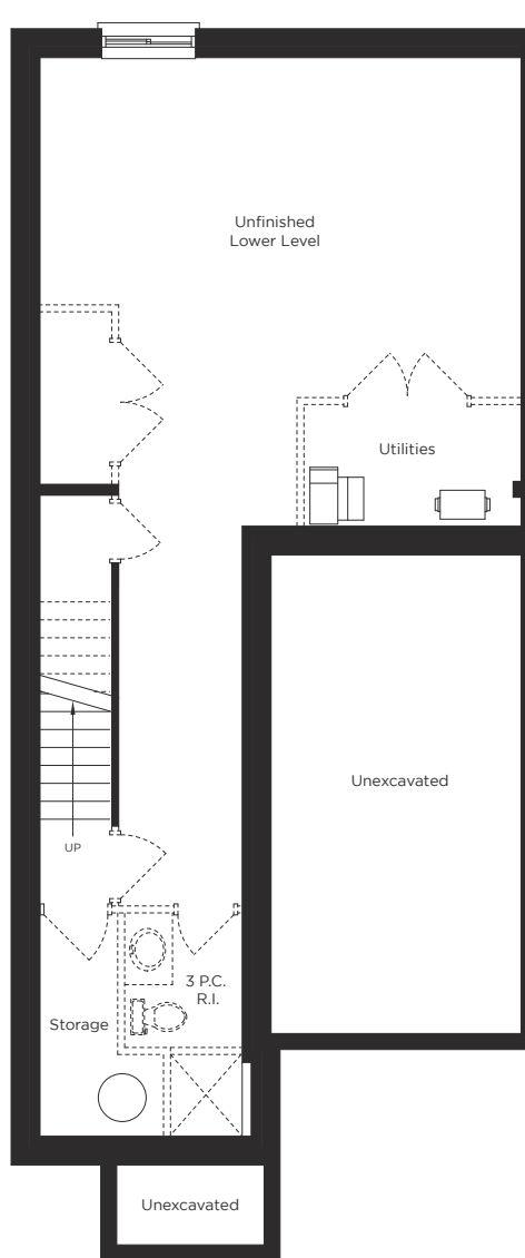
BASEMENT
