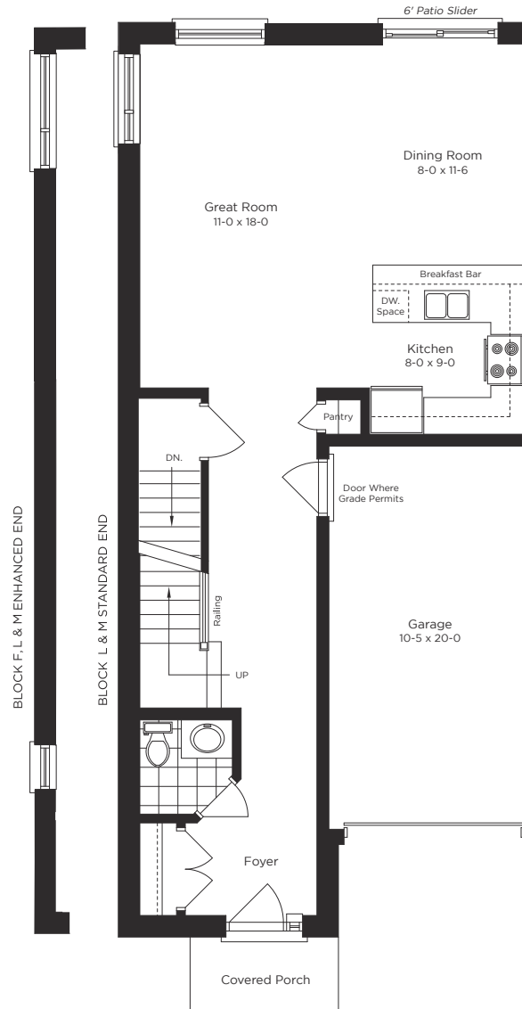
MAIN FLOOR
